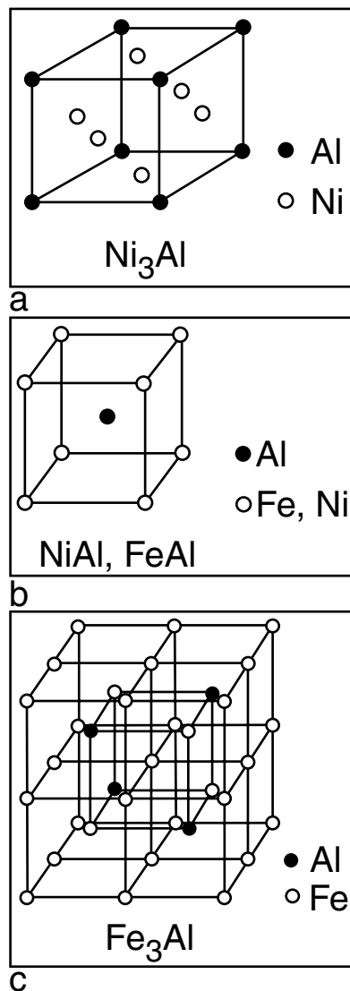
FIGURE A.3 The crystal structure of nickel and iron aluminides: (a) \text{L1}_2 , (b) \text{B}_2 , (c) \text{DO}_3 . (From Schwartz, M., Emerging Technology , Technomics, 19. With permission.)
