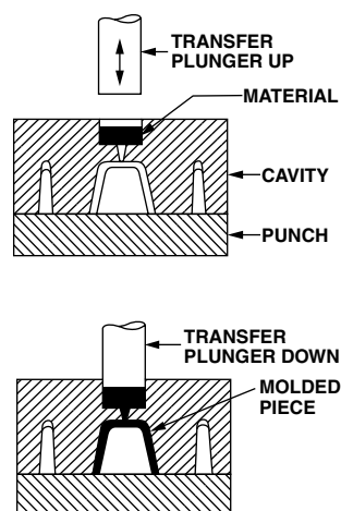
FIGURE C.5 Transfer molding.
