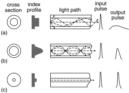
FIGURE O.1 Types of optical fiber designs. (a) Multimode, stepped-refractive-index profile. (b) Multimode, graded-index profile. (c) Single-mode, stepped-index. Graded index is possible. (From McGraw-Hill Encyclopedia of Science and Technology , 8th ed., Vol. 12, 431. With permission.)
