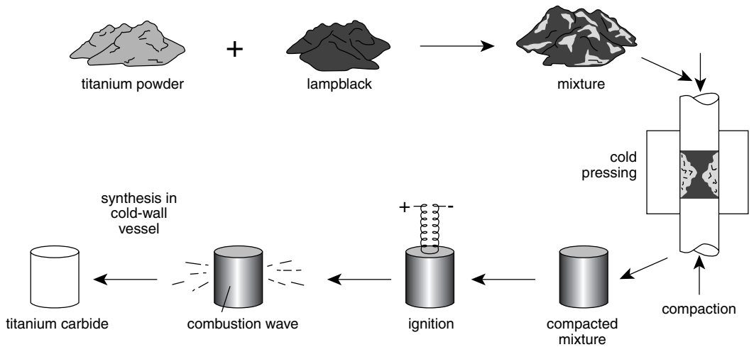
FIGURE M.6 Illustration of self-propagating, high-temperature synthesis. (From McGraw-Hill Handbook of Structural Ceramics , McGraw-Hill, New York, 1992, 423. With permission.)
