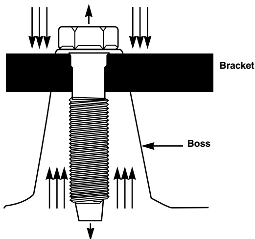
FIGURE F.1 Features of a bolt. (From Adv. Mater. Proc. , 154(4), 49, 1998. with permission.)
