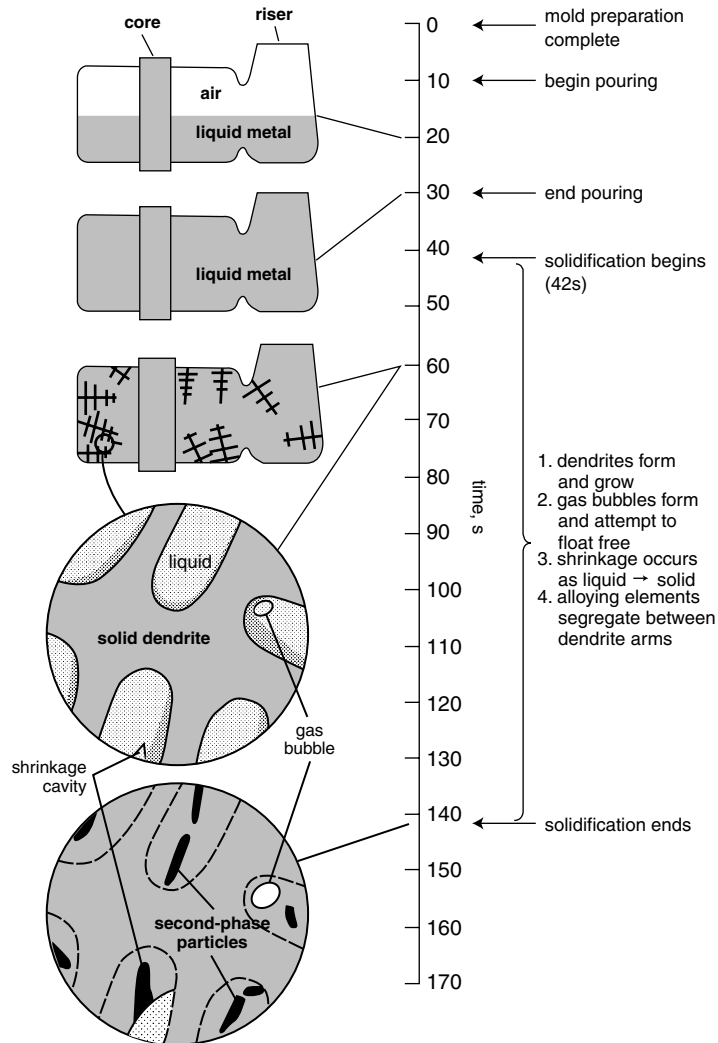
FIGURE M.9 Solidification and processing for a cast-to-shape part. (From McGraw-Hill Encyclopedia of Science and Technology , 8th ed., Vol. 11, McGraw-Hill, New York, 35. With permission.)
