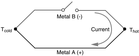
FIGURE T.2 Schematic drawing of a thermocouple.
